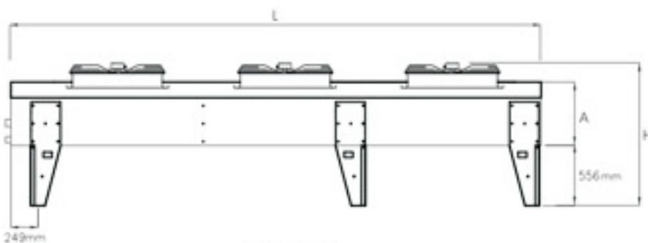
FRONT VIEW
